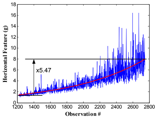
Figure 9. Plot of horizontal feature for bearing 1_1 from the time of anomaly to the end of the first degradation mode. Exponential curve fit is shown.
